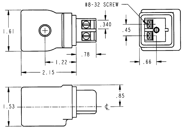
S100, S200, S300-Screw Terminations
