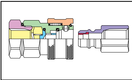
Disconnected: Valve in coupler shuts gas off (QD valve should not be the only means to shut gas supply off over an extended period of time. A gas shut-off valve should be installed before the coupler for extended periods).
